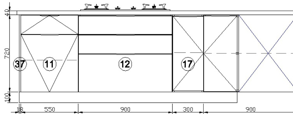
D View elevation drawing
