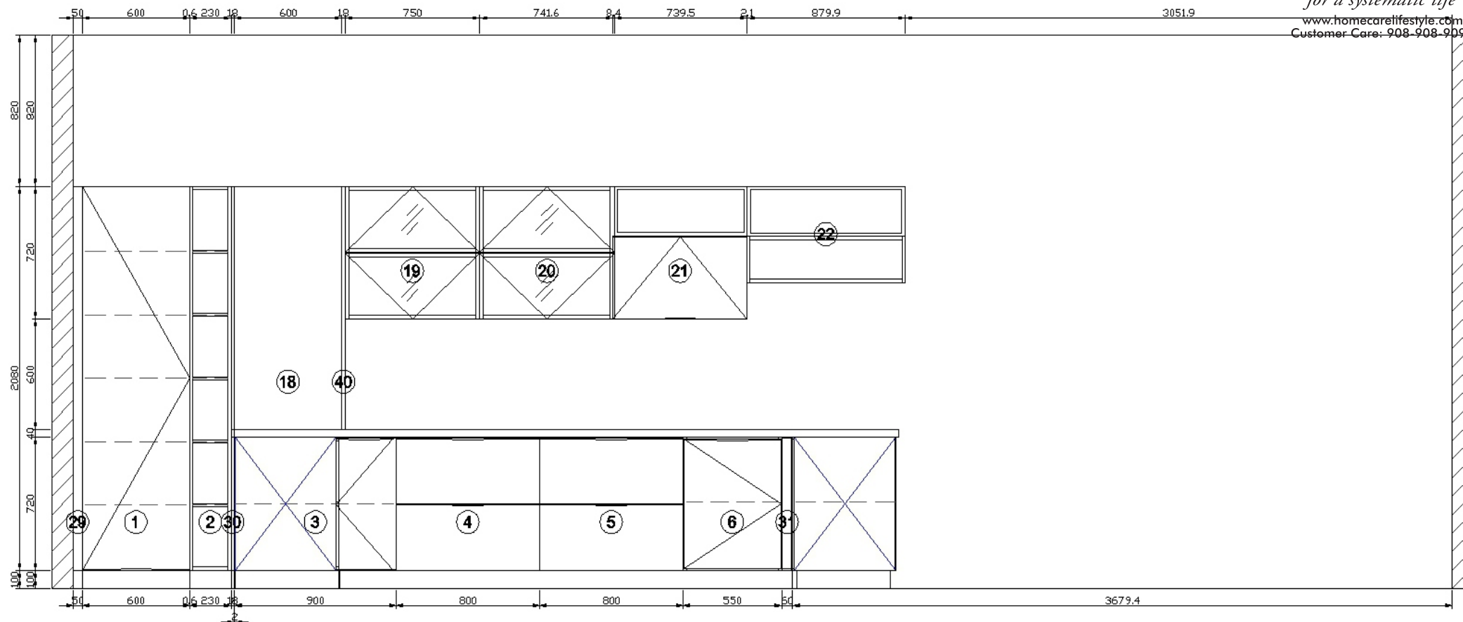
A View elevation drawing
